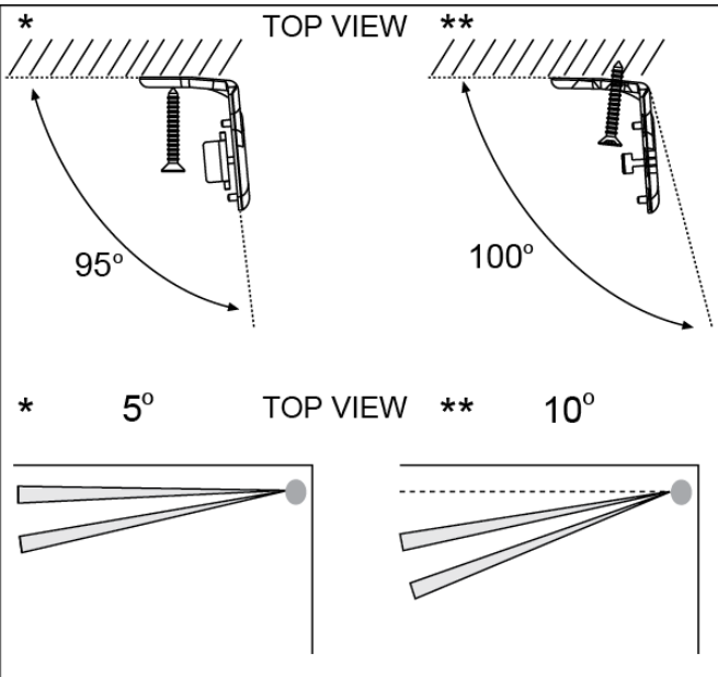
Figure 11. Mounting Bracket to Surface
