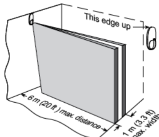
Figure 2. Wall-Mount Curtain
