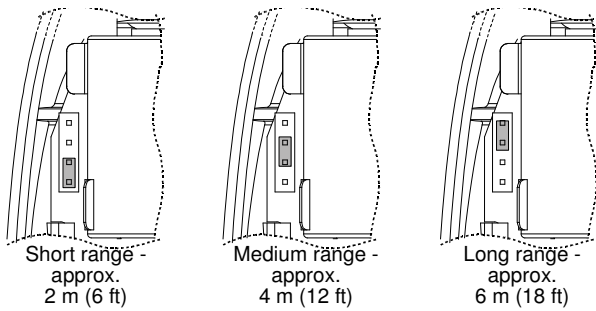
Figure 15. Range Jumper Settings
