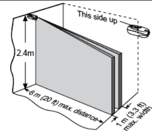
Figure 3. Ceiling-Mount Curtain
