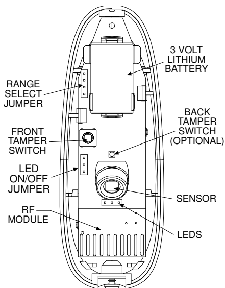
Figure 7. Internal View
