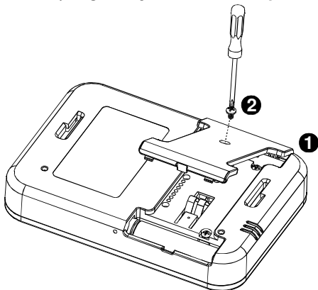
Figure 2 - Battery Cover Mounting (part a)
